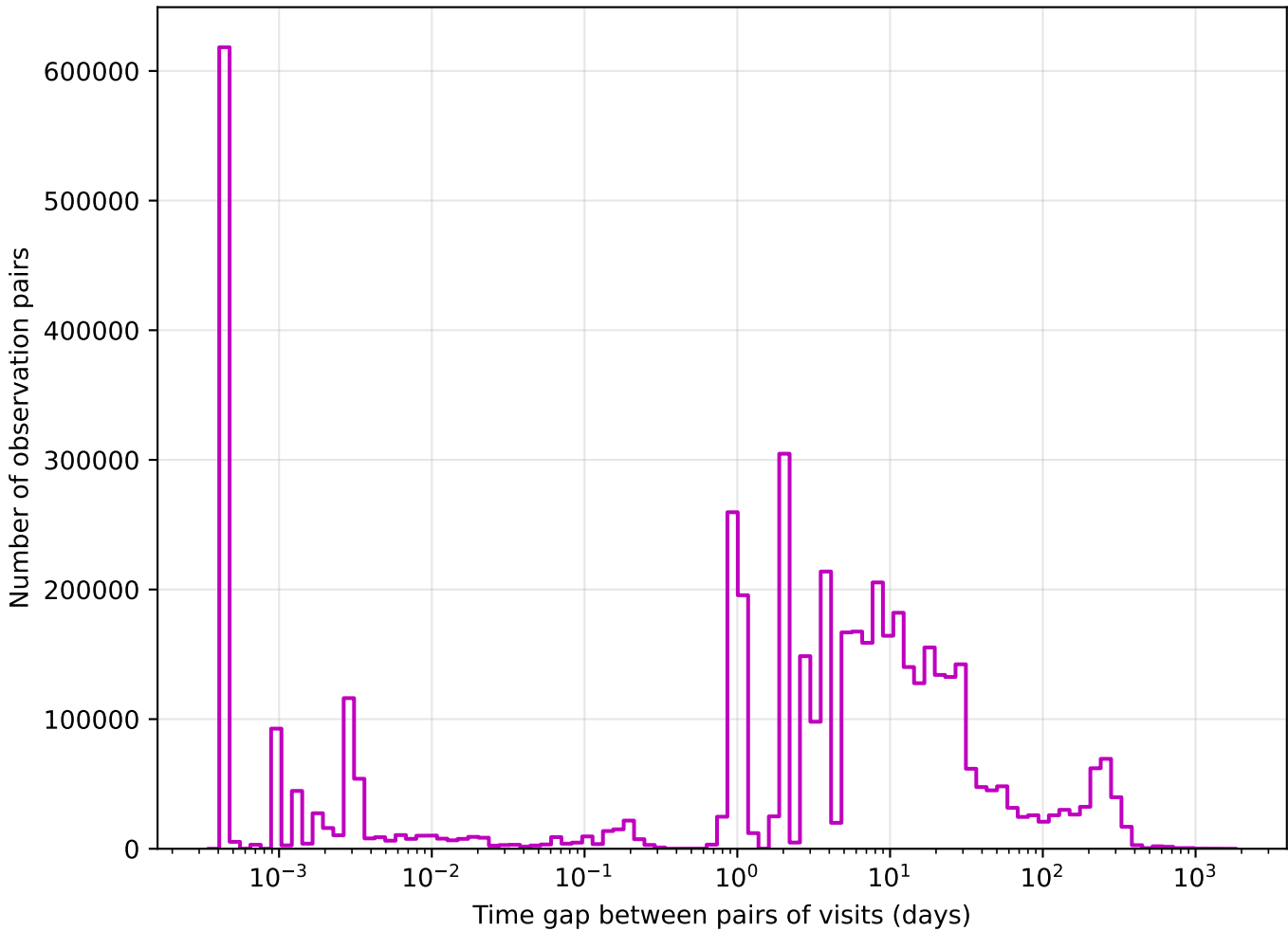
weather_cloudso14v3.4_10yrs z band: Tgaps observationStartMJD
