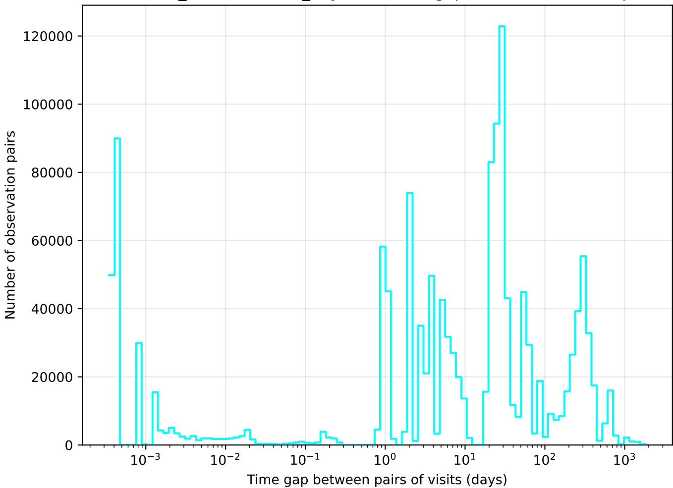
weather_cloudso14v3.4_10yrs u band: Tgaps observationStartMJD
