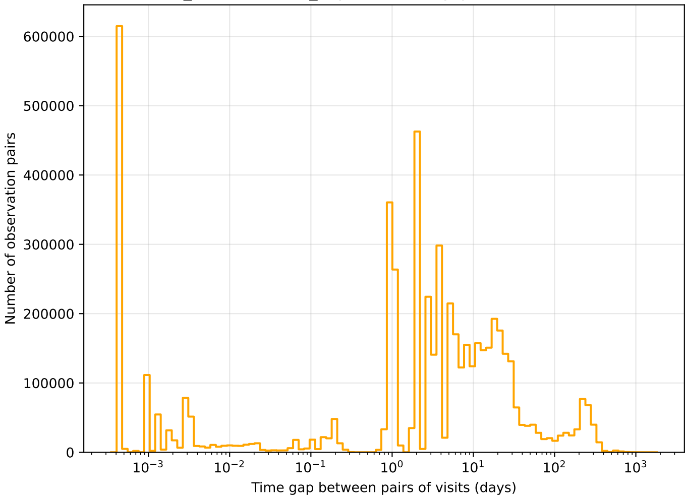
weather_cloudso14v3.4_10yrs r band: Tgaps observationStartMJD
