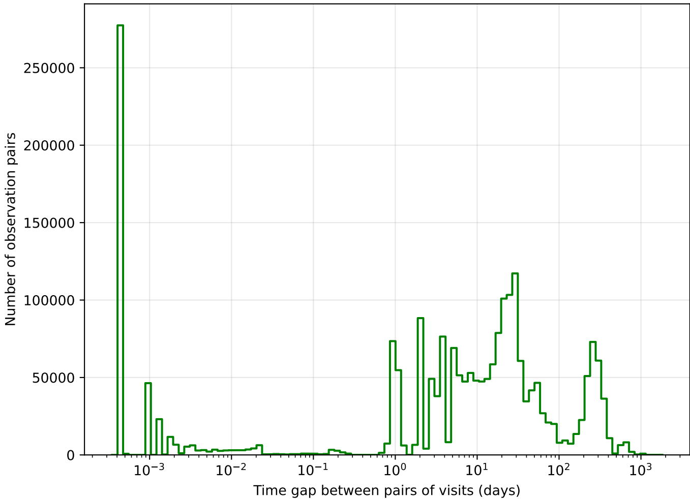
weather_cloudso14v3.4_10yrs g band: Tgaps observationStartMJD
