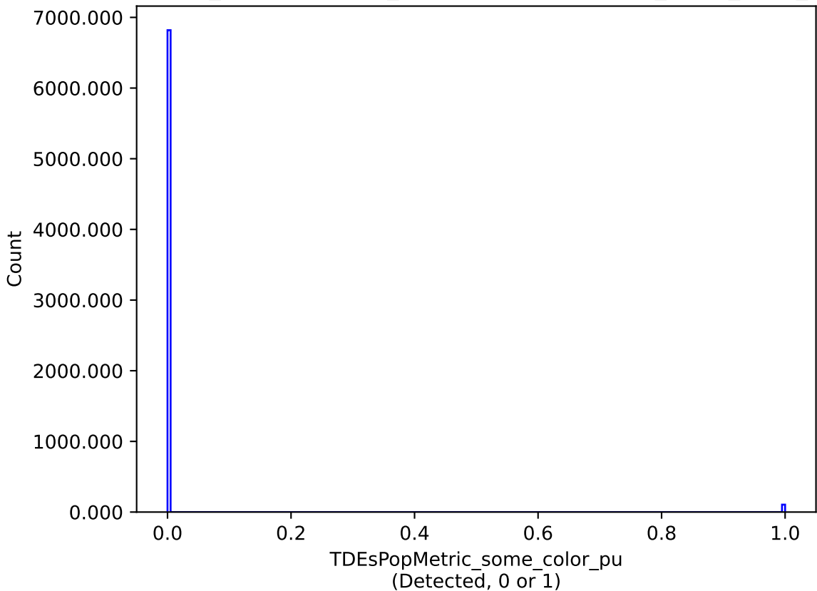
weather_cloudso14v3.4_10yrs : TDEsPopMetric_some_color_pu
