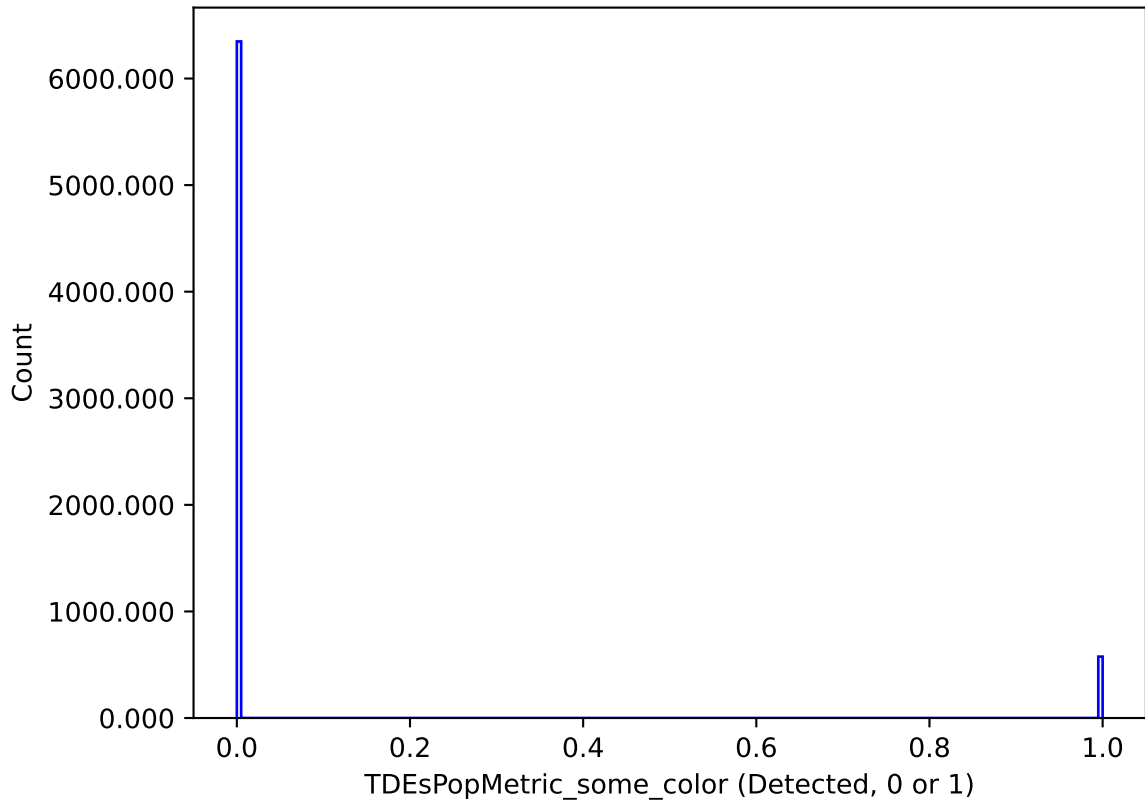
weather_cloudso14v3.4_10yrs : TDEsPopMetric_some_color
