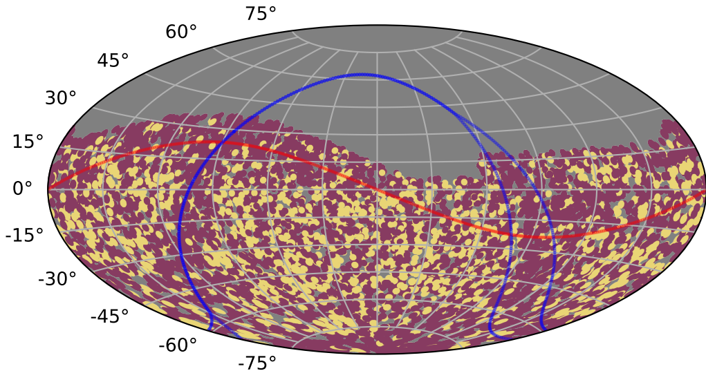
weather_cloudso14v3.4_10yrs : TDEsPopMetric_prepeak
