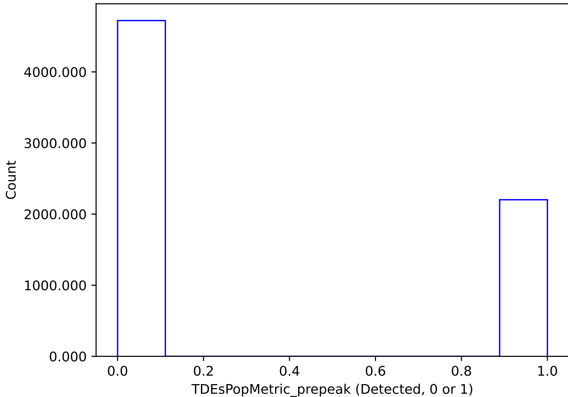
weather_cloudso14v3.4_10yrs : TDEsPopMetric_prepeak
