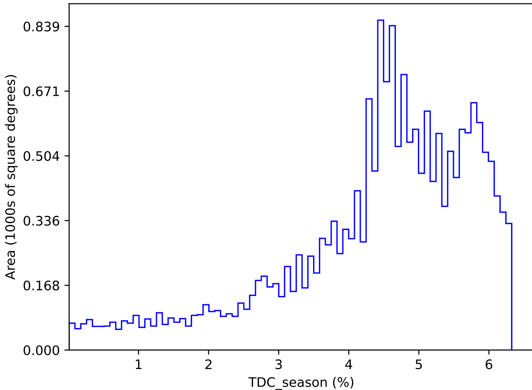
weather_cloudso14v3.4_10yrs : TDC_season
