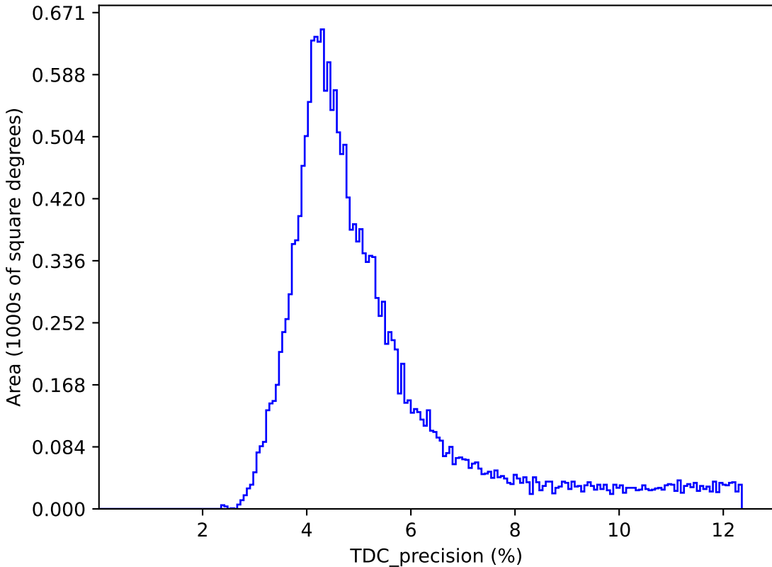
weather_cloudso14v3.4_10yrs : TDC_precision
