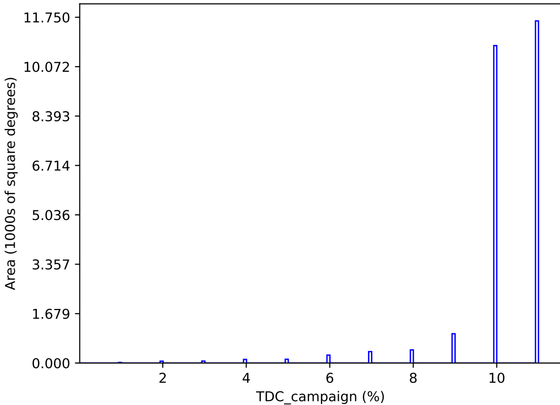
weather_cloudso14v3.4_10yrs : TDC_campaign
