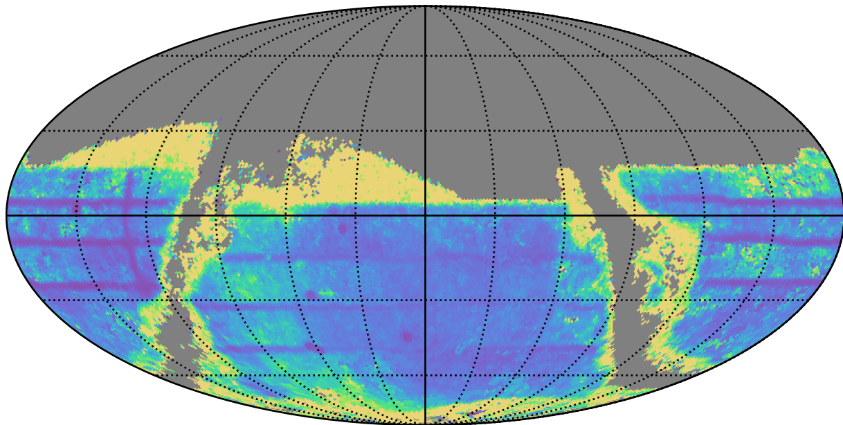
weather_cloudso14v3.4_10yrs : TDC_cadence
