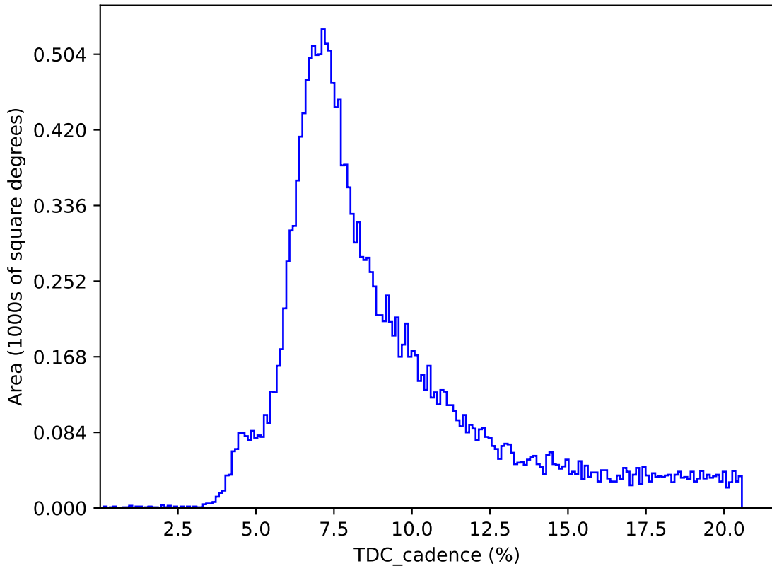
weather_cloudso14v3.4_10yrs : TDC_cadence
