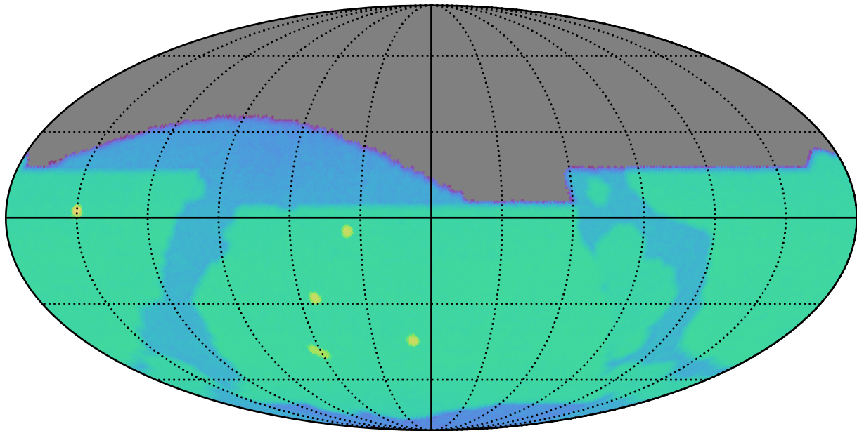
weather_cloudso14v3.4_10yrs z: SurfaceBrightLimit
