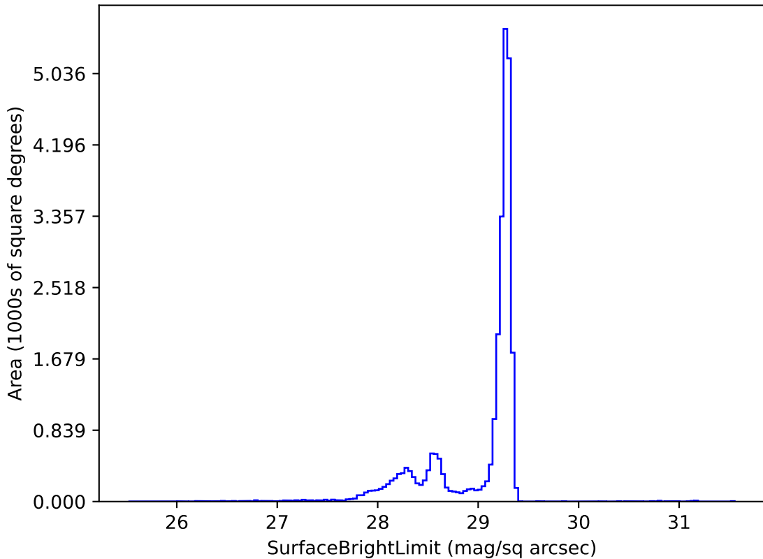
weather_cloudso14v3.4_10yrs z: SurfaceBrightLimit
