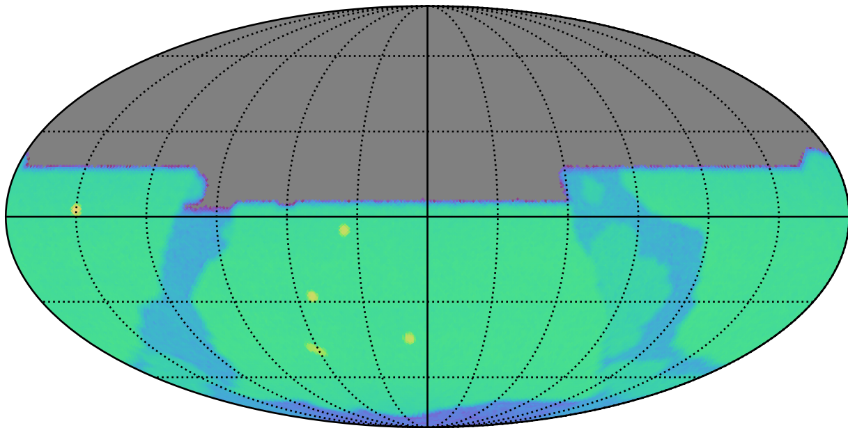
weather_cloudso14v3.4_10yrs y: SurfaceBrightLimit
