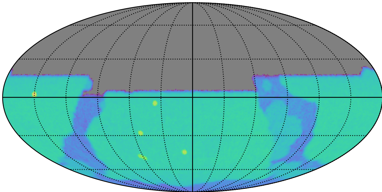
weather_cloudso14v3.4_10yrs u: SurfaceBrightLimit
