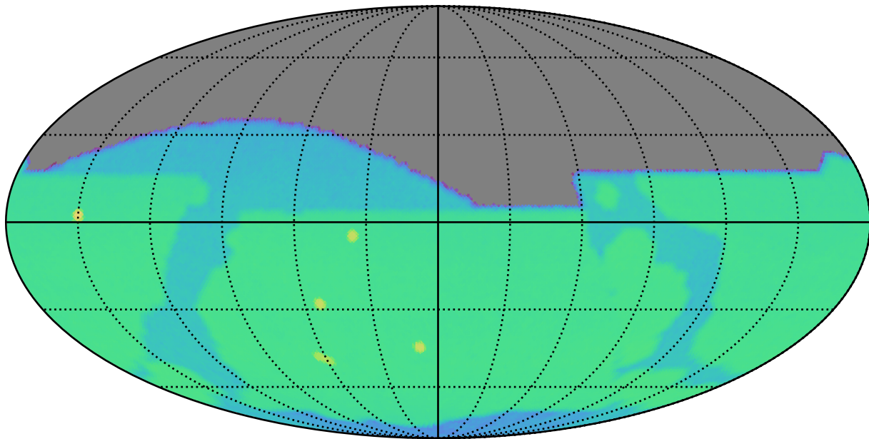
weather_cloudso14v3.4_10yrs r: SurfaceBrightLimit
