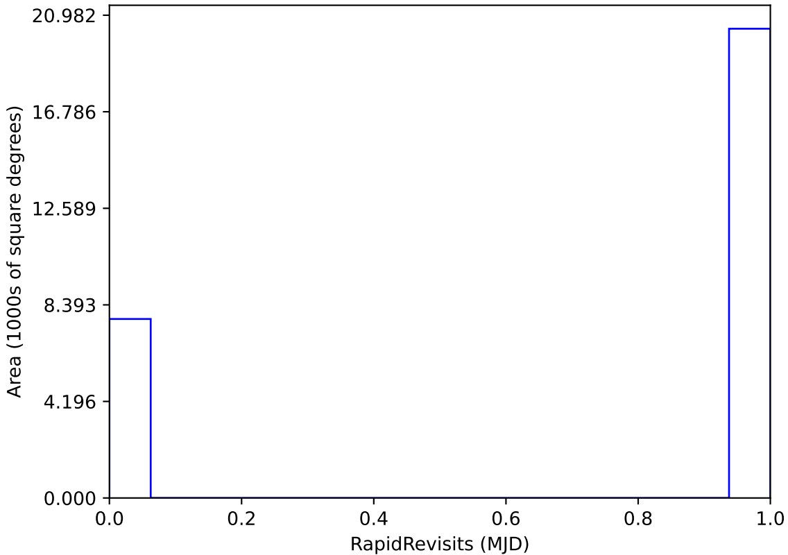
weather_cloudso14v3.4_10yrs : RapidRevisits
