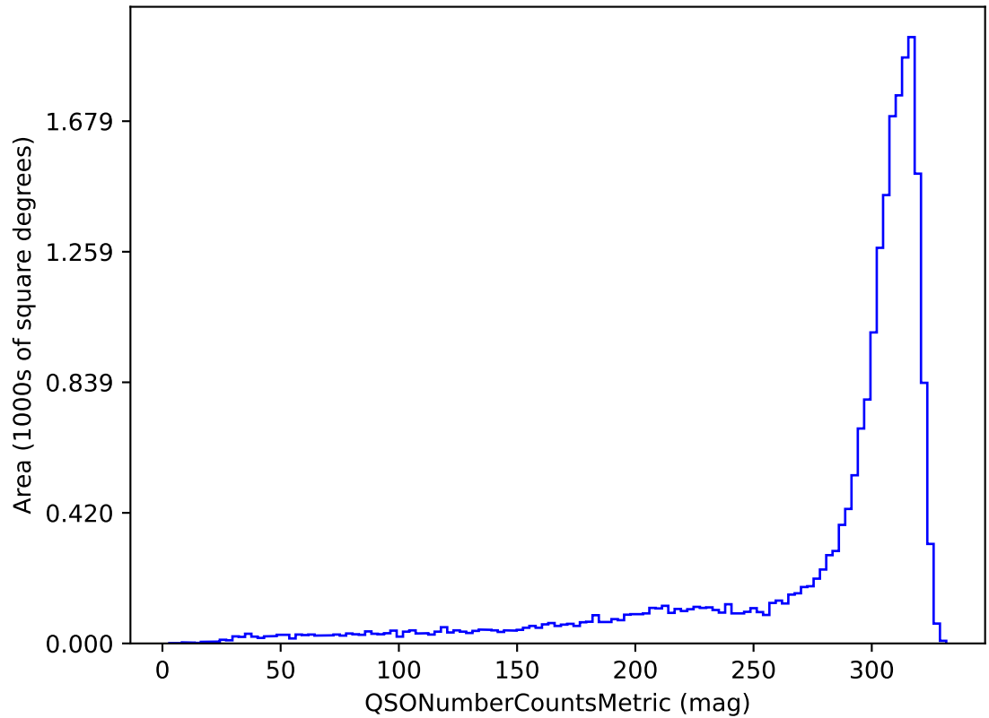
weather_cloudso14v3.4_10yrs u band and non-DD: QSONumberCountsMetric
