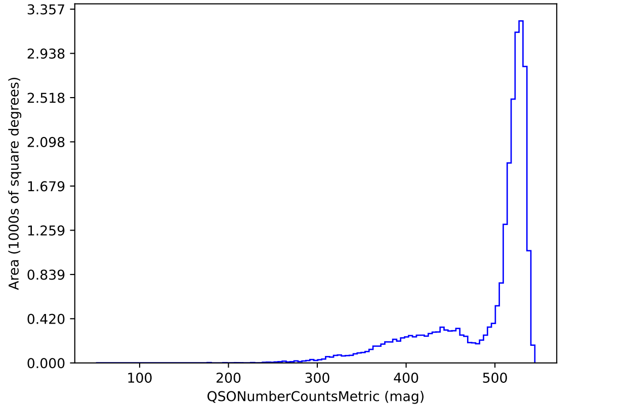
weather_cloudso14v3.4_10yrs r band and non-DD: QSONumberCountsMetric
