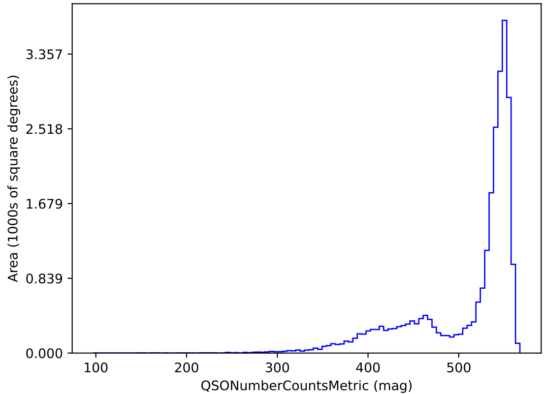
weather_cloudso14v3.4_10yrs i band and non-DD: QSONumberCountsMetric
