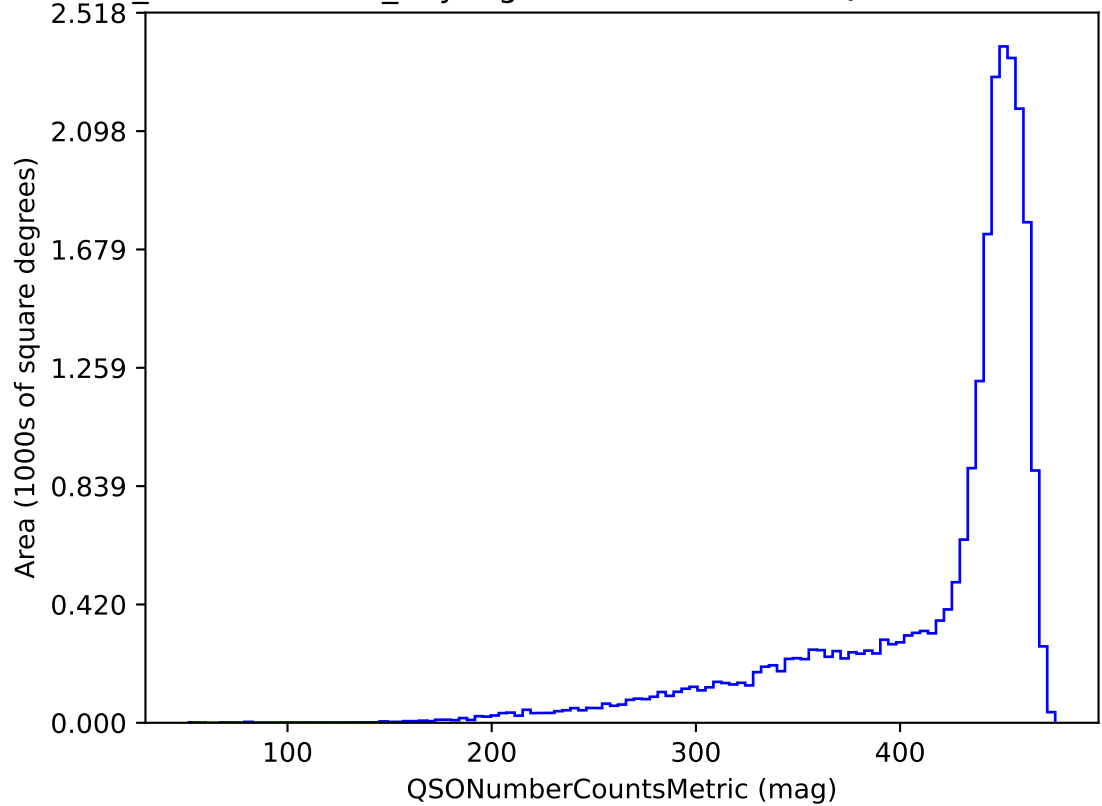
weather_cloudso14v3.4_10yrs g band and non-DD: QSONumberCountsMetric
