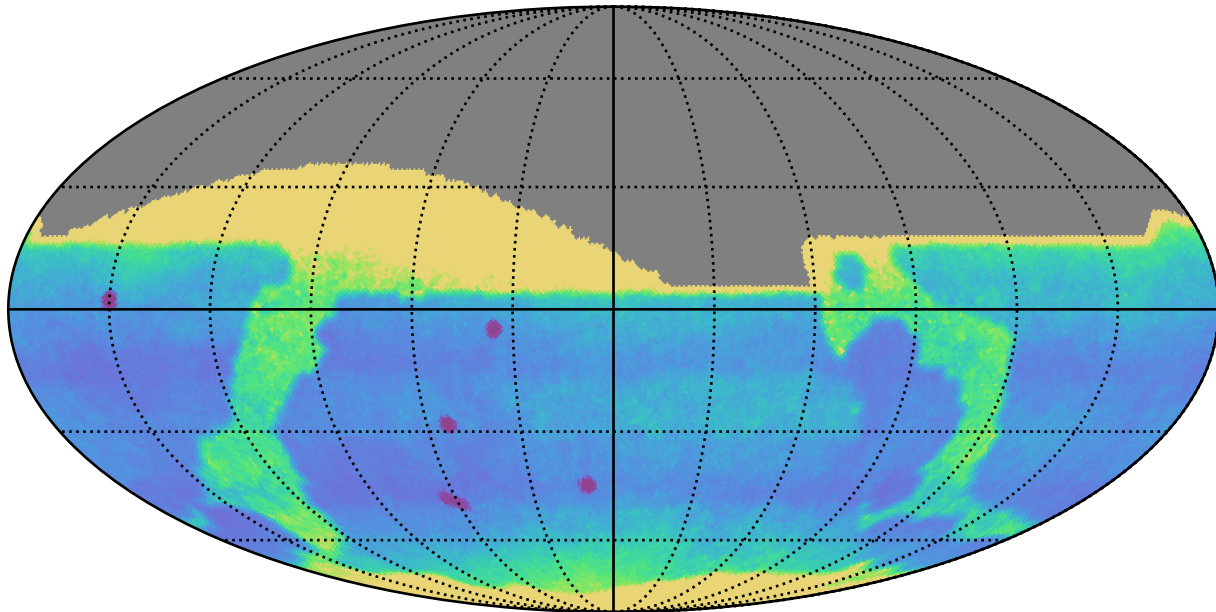
weather_cloudso14v3.4_10yrs : Proper Motion Uncert @ 24.0
