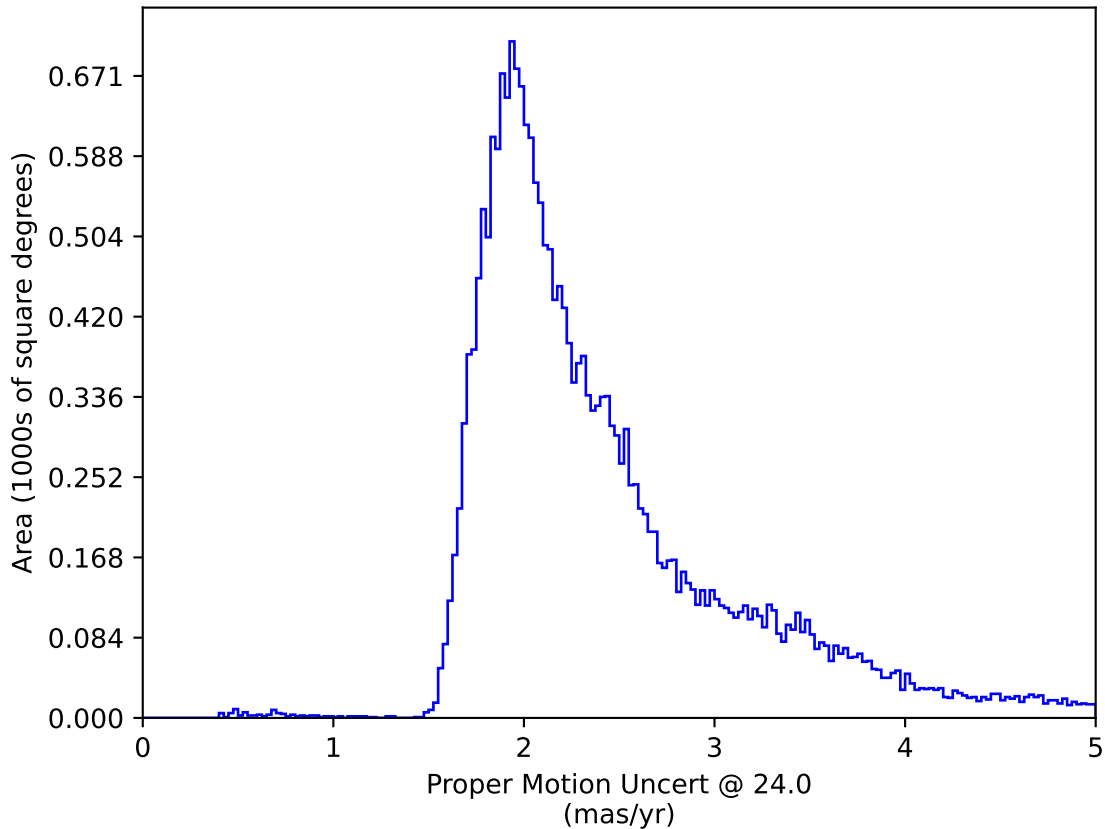
weather_cloudso14v3.4_10yrs : Proper Motion Uncert @ 24.0
