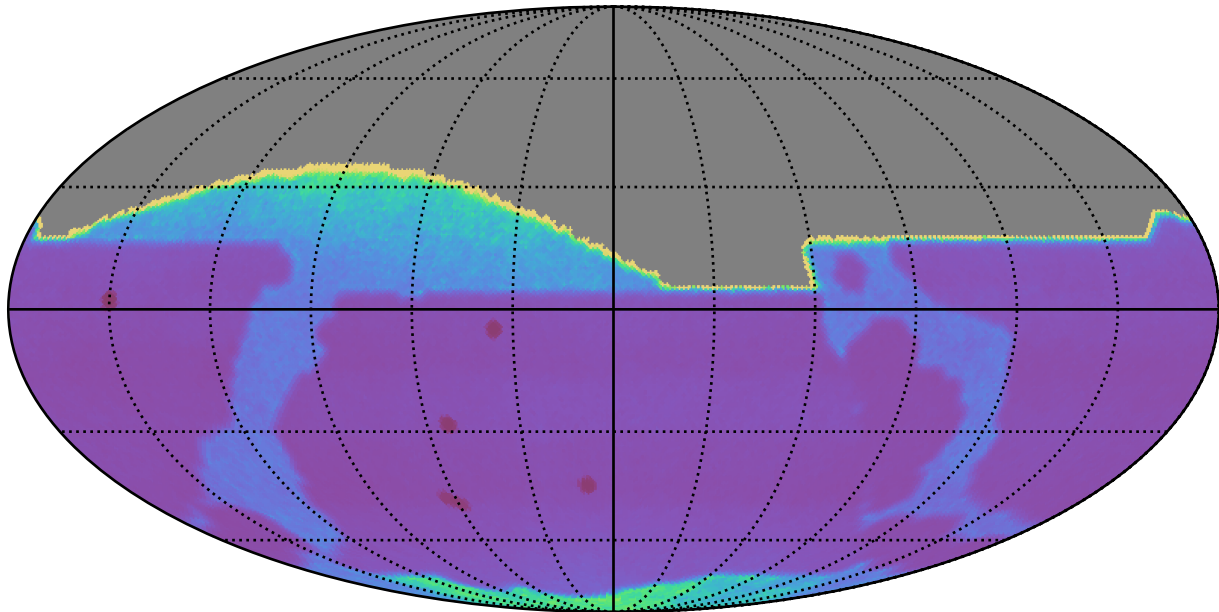
weather_cloudso14v3.4_10yrs : Proper Motion Uncert @ 20.5
