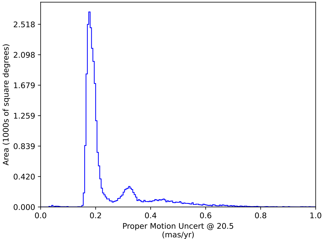
weather_cloudso14v3.4_10yrs : Proper Motion Uncert @ 20.5
