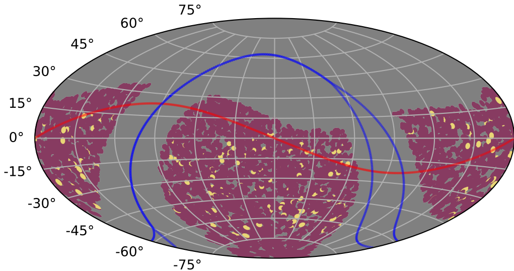
weather_cloudso14v3.4_10yrs : PrestoKNe_score_s
