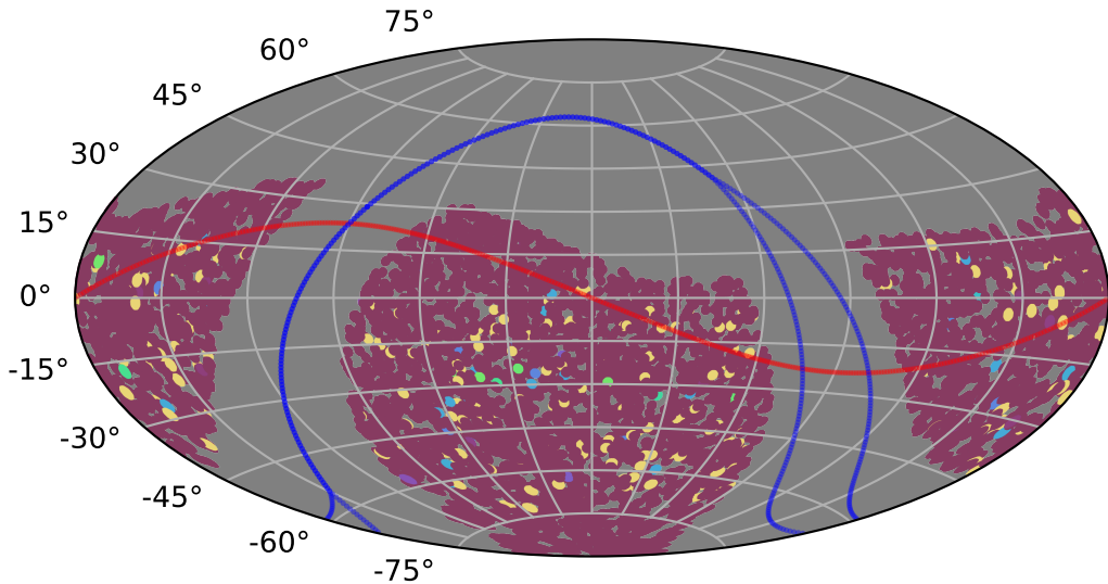
weather_cloudso14v3.4_10yrs : PrestoKNe_score_p
