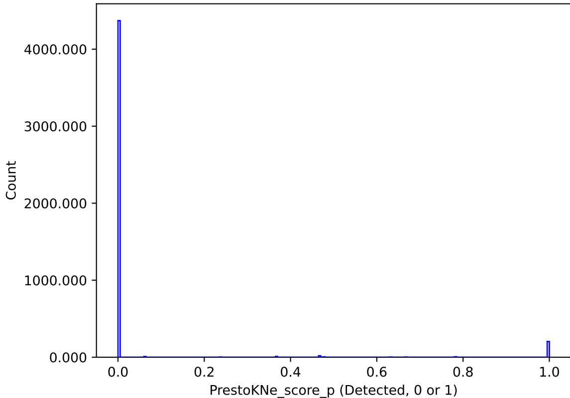
weather_cloudso14v3.4_10yrs : PrestoKNe_score_p
