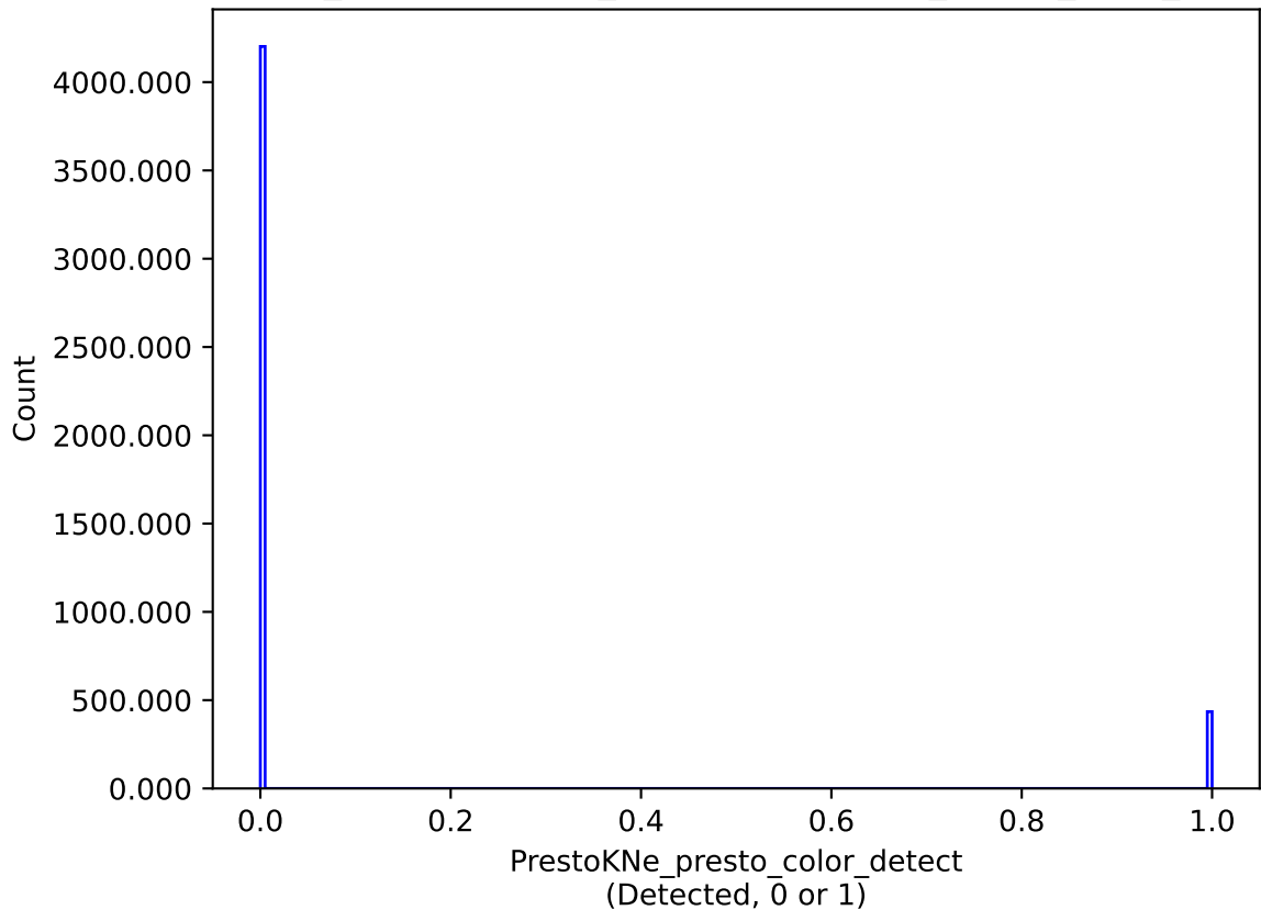
weather_cloudso14v3.4_10yrs : PrestoKNe_presto_color_detect
