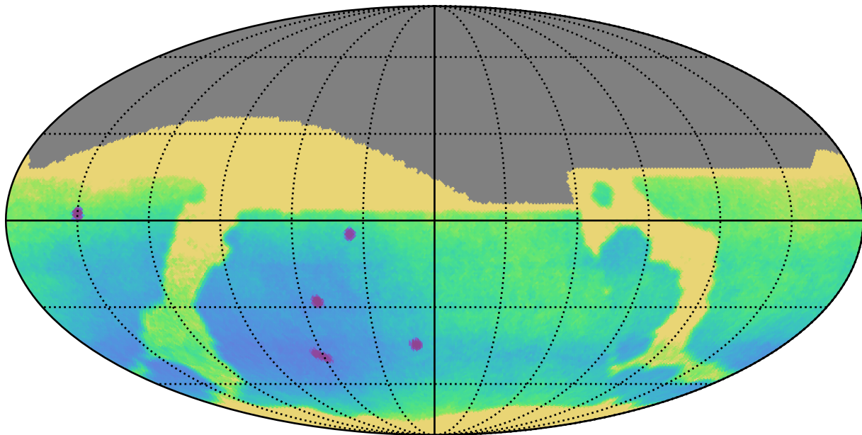
weather_cloudso14v3.4_10yrs : Parallax Uncert @ 24.0
