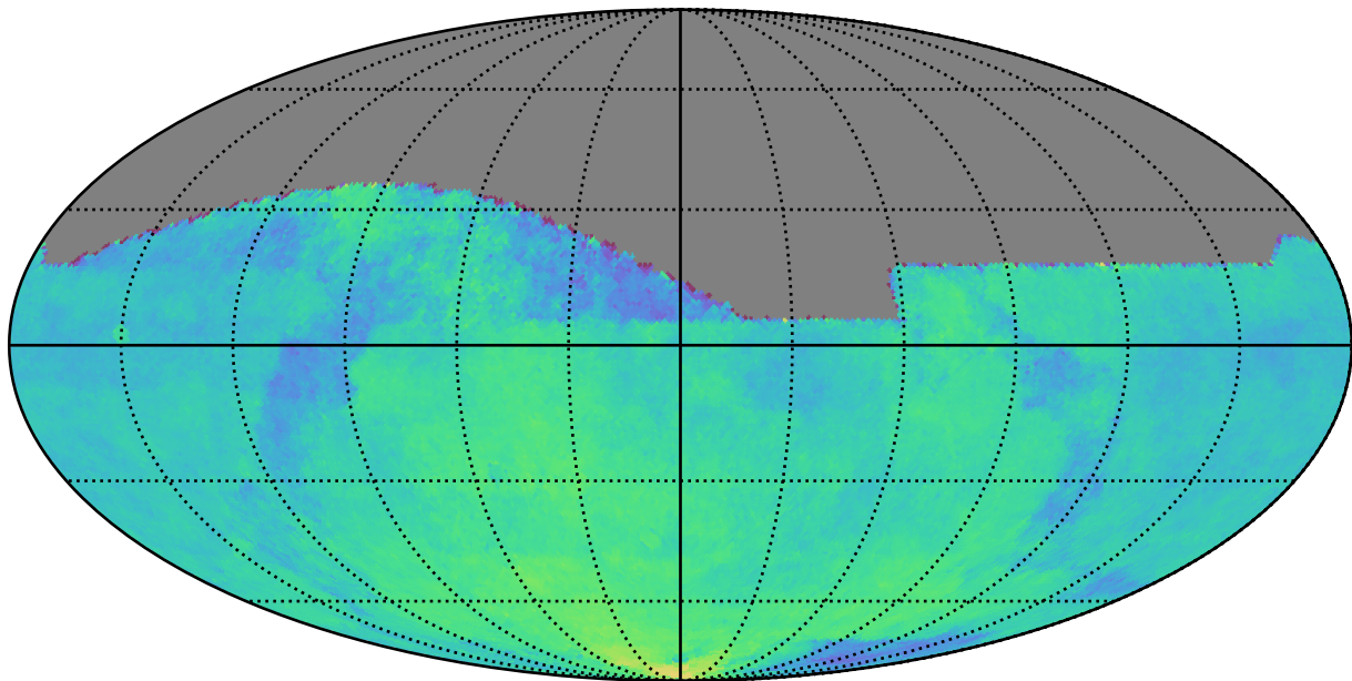
weather_cloudso14v3.4_10yrs : Parallax Coverage @ 24.0
