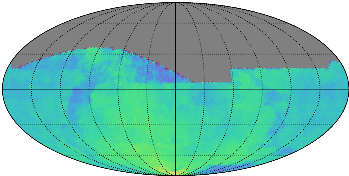
weather_cloudso14v3.4_10yrs : Parallax Coverage @ 22.4
