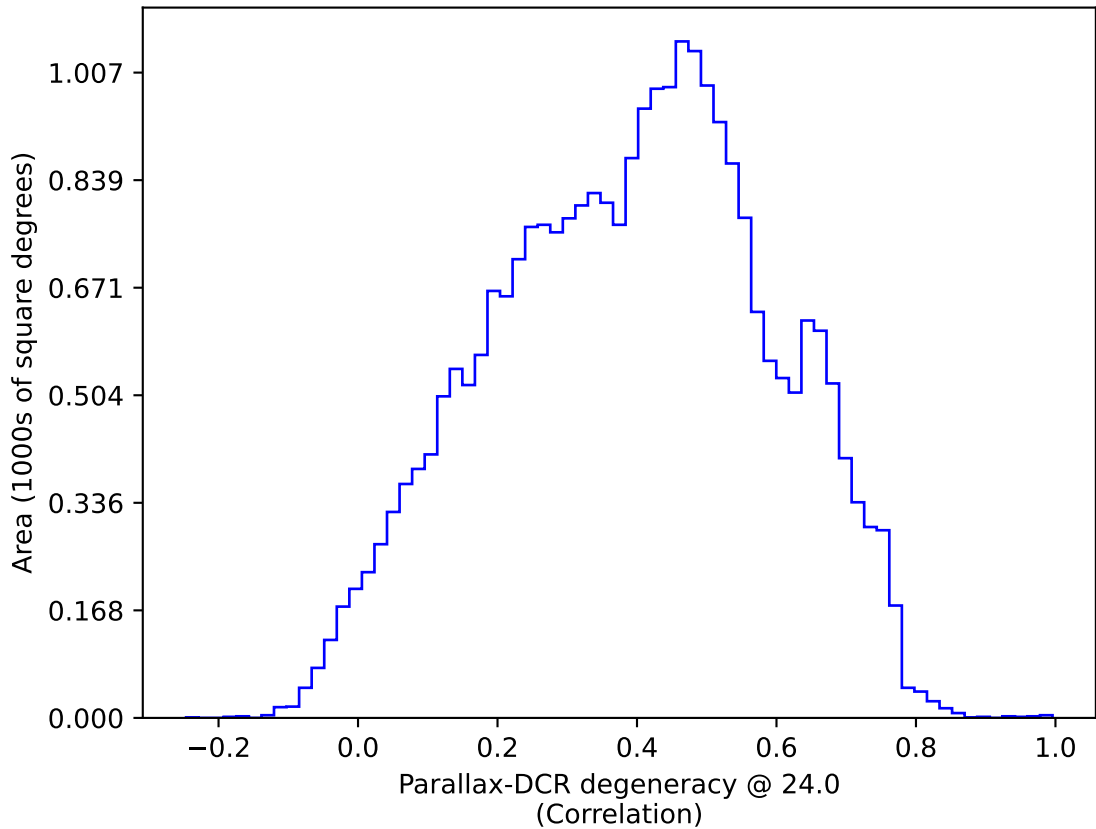
weather_cloudso14v3.4_10yrs : Parallax-DCR degeneracy @ 24.0
