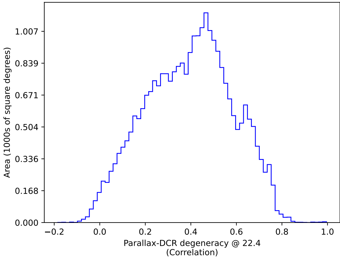
weather_cloudso14v3.4_10yrs : Parallax-DCR degeneracy @ 22.4
