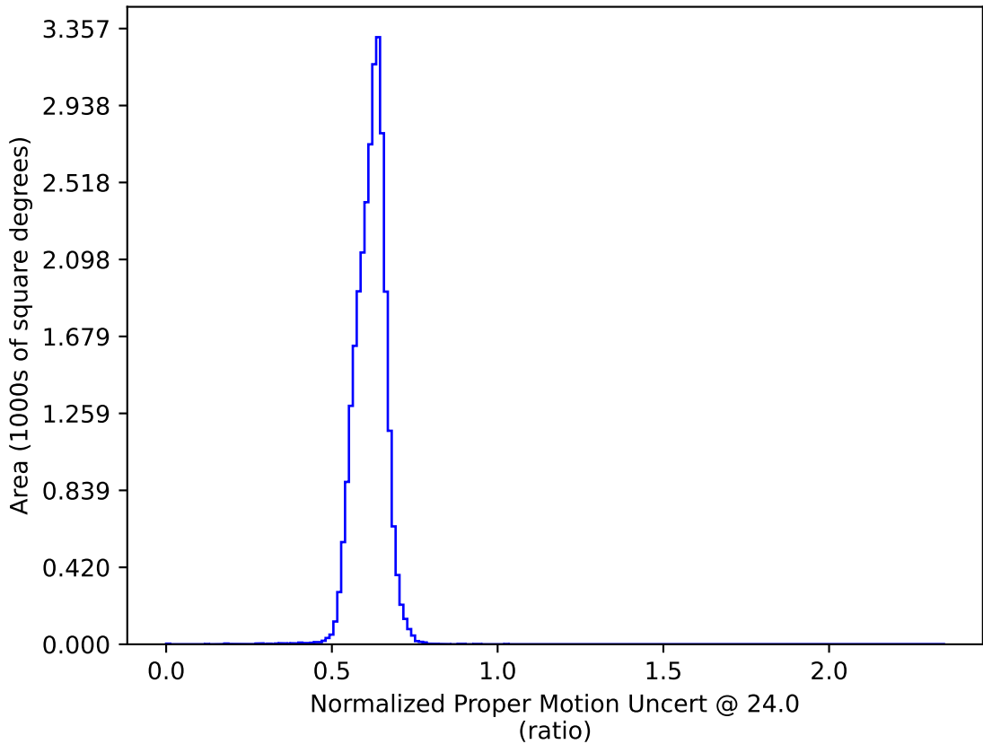
weather_cloudso14v3.4_10yrs : Normalized Proper Motion Uncert @ 24.0
