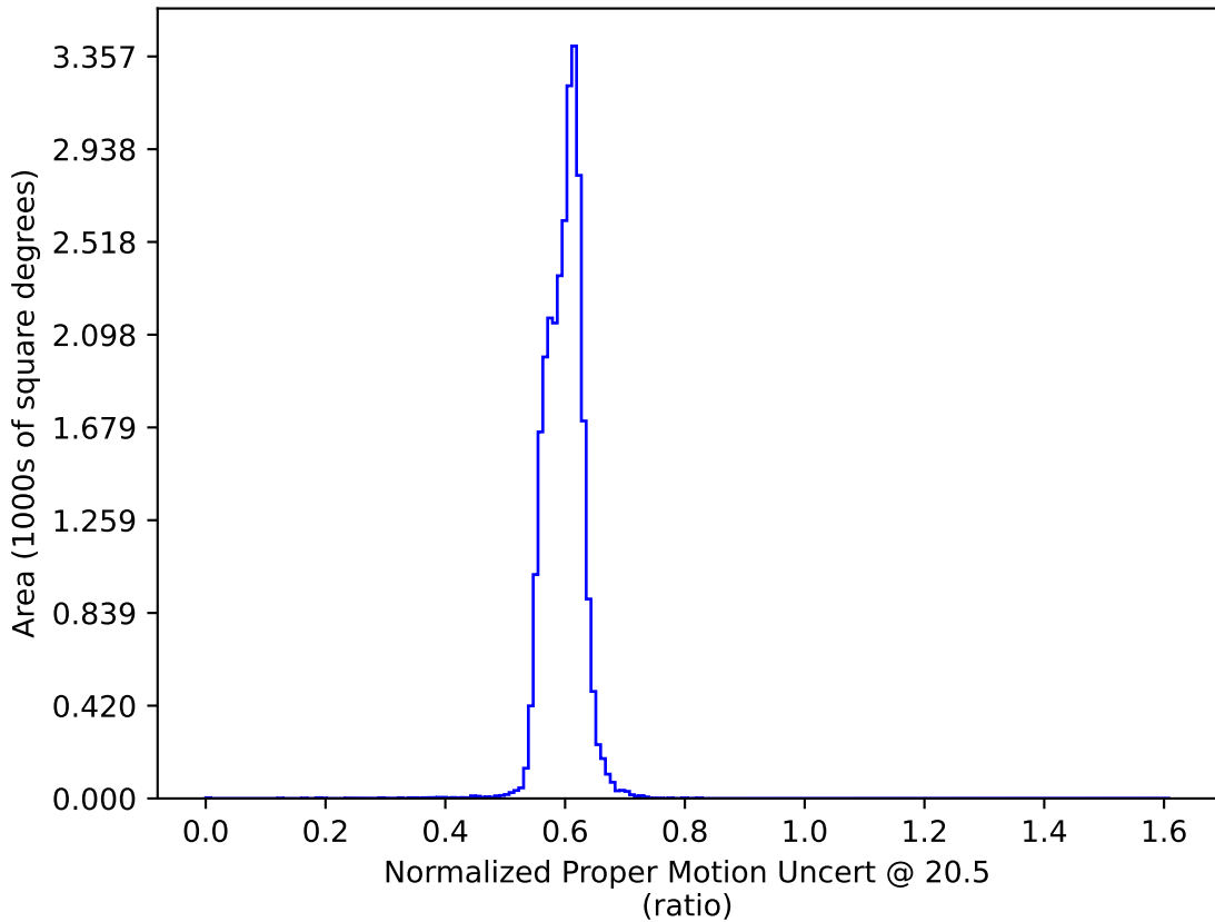
weather_cloudso14v3.4_10yrs : Normalized Proper Motion Uncert @ 20.5
