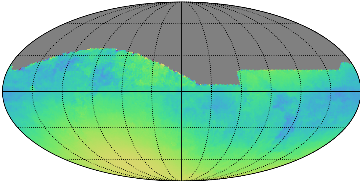
weather_cloudso14v3.4_10yrs : Normalized Parallax Uncert @ 24.0
