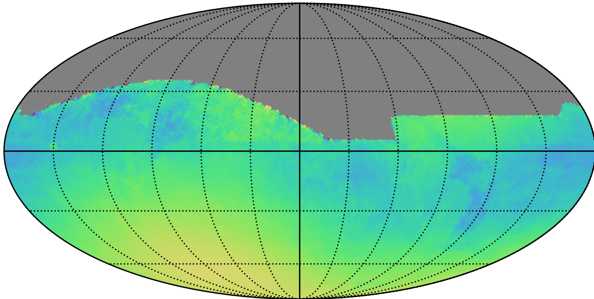
weather_cloudso14v3.4_10yrs : Normalized Parallax Uncert @ 22.4
