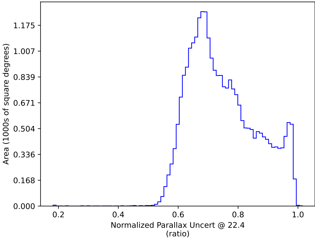
weather_cloudso14v3.4_10yrs : Normalized Parallax Uncert @ 22.4
