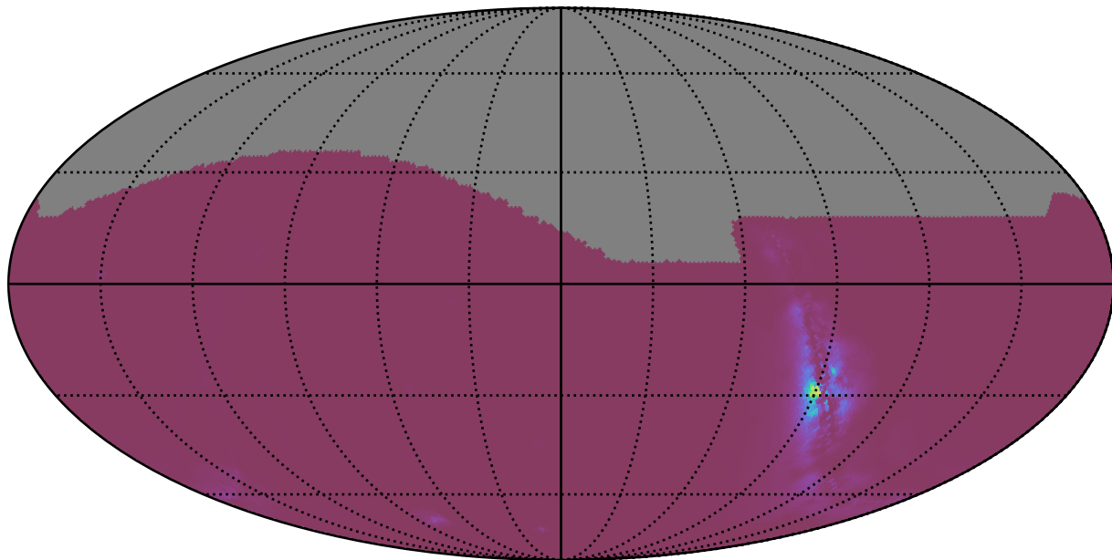
weather_cloudso14v3.4_10yrs : NlcPoints
