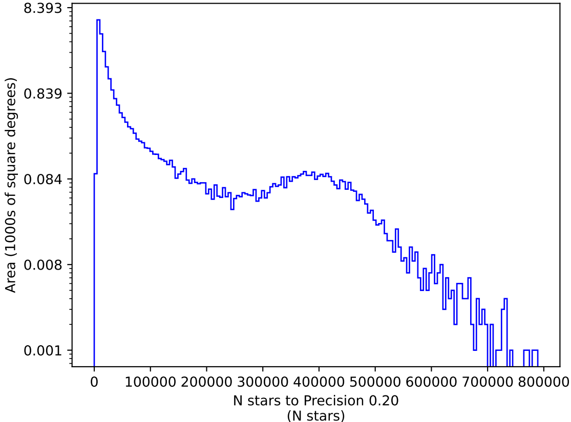
weather_cloudso14v3.4_10yrs z: N stars to Precision 0.20
