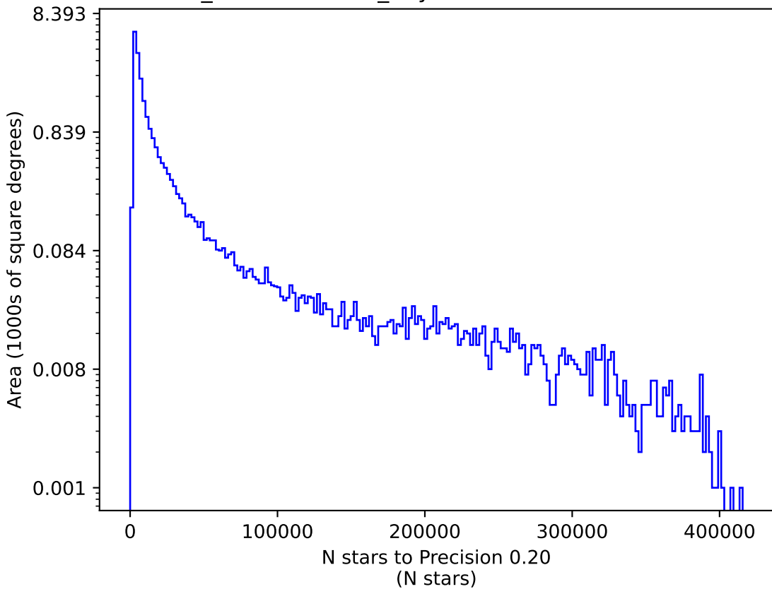
weather_cloudso14v3.4_10yrs u: N stars to Precision 0.20
