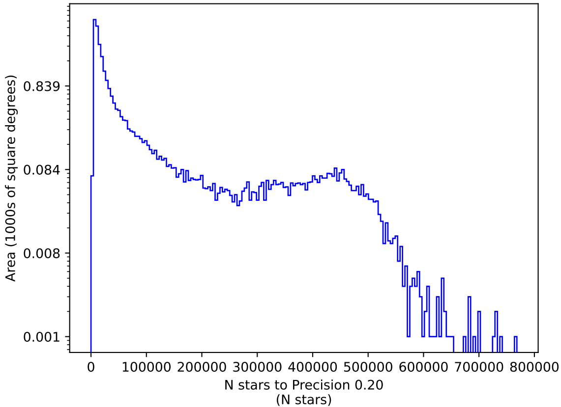
weather_cloudso14v3.4_10yrs r: N stars to Precision 0.20
