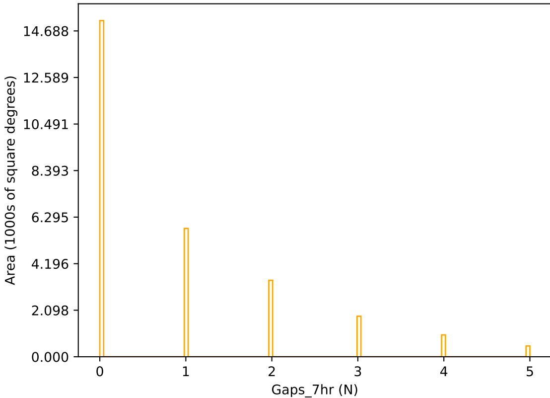
weather_cloudso14v3.4_10yrs r band: Gaps_7hr
