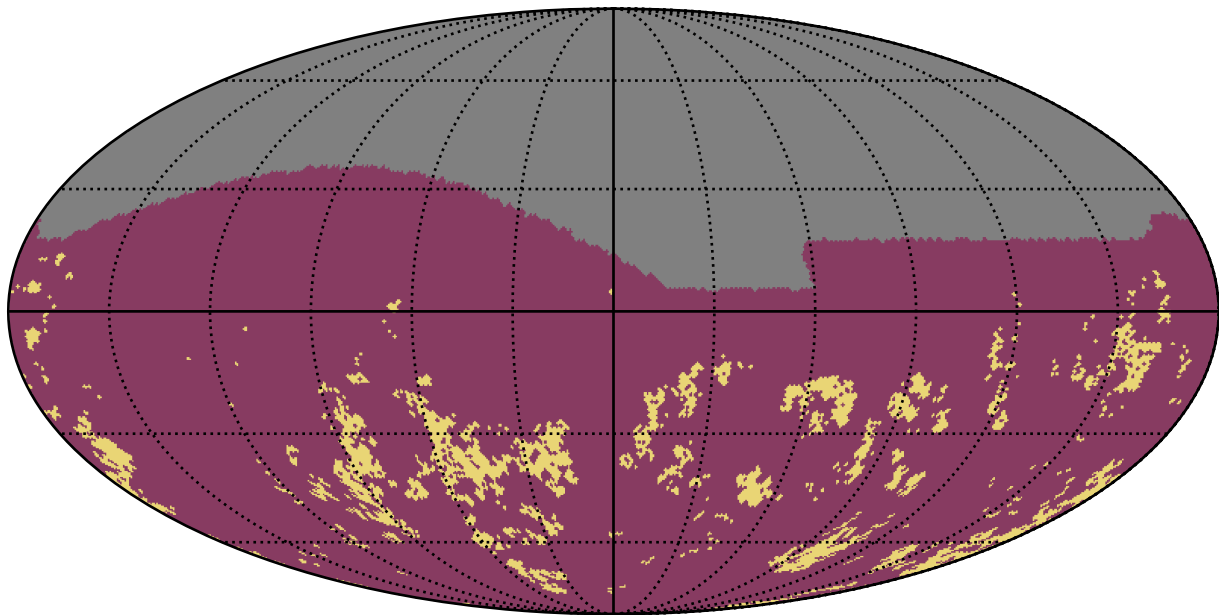
weather_cloudso14v3.4_10yrs g band: Gaps_7hr
