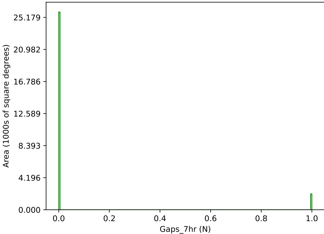
weather_cloudso14v3.4_10yrs g band: Gaps_7hr
