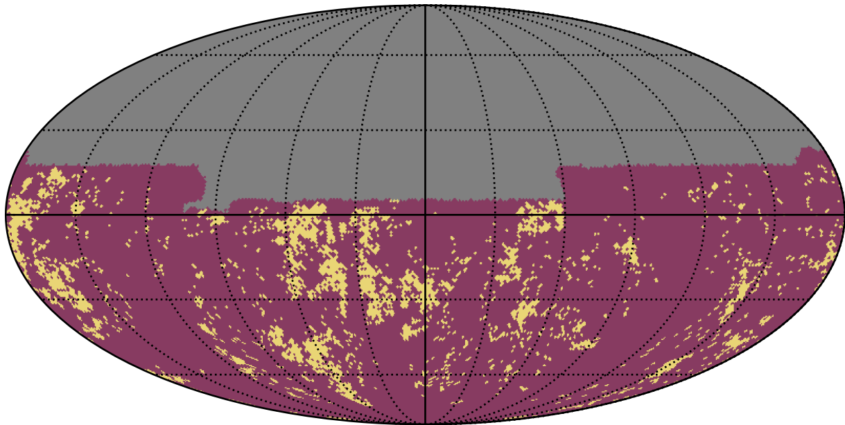
weather_cloudso14v3.4_10yrs u band: Gaps_3hr
