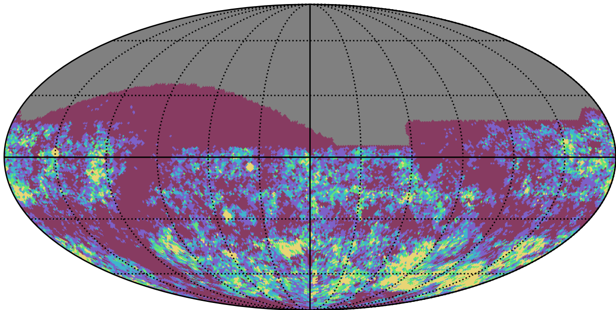
weather_cloudso14v3.4_10yrs i band: Gaps_3hr
